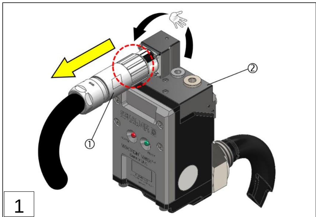
1: Hybrid connector
