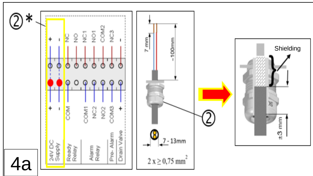
Fig.: 46 : VN301 plus central unit; establish power supply (connect contacts)
