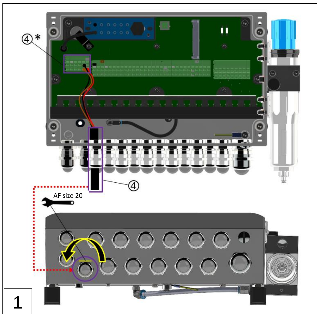
Fig.: 65 : VN301 plus central unit; establish communication with Remote Indicator II (optional)
