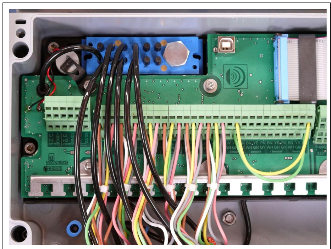
Fig.: 55 : Assembly and installation complete (steps 1 - 7; example with 6 hybrid hoses)
