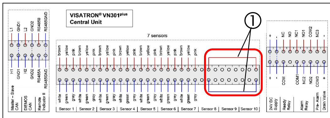
Fig.: 61 : VN301 plus central unit: Configuration of the wiring bridges; 7 sensors
