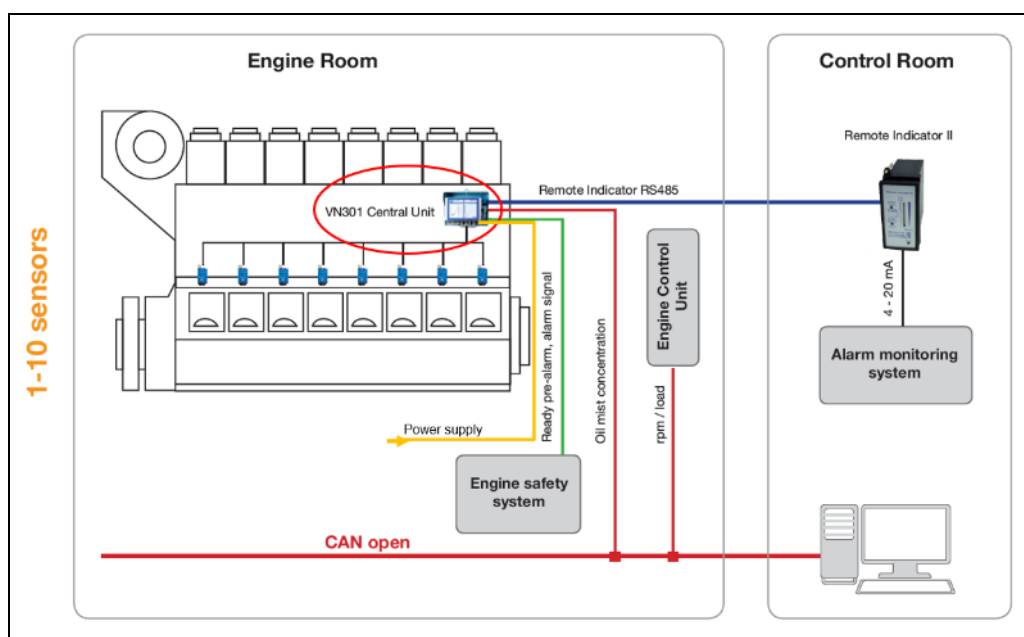
Fig.: 33 : Operating mode 1 "Master", VN301 plus central unit
